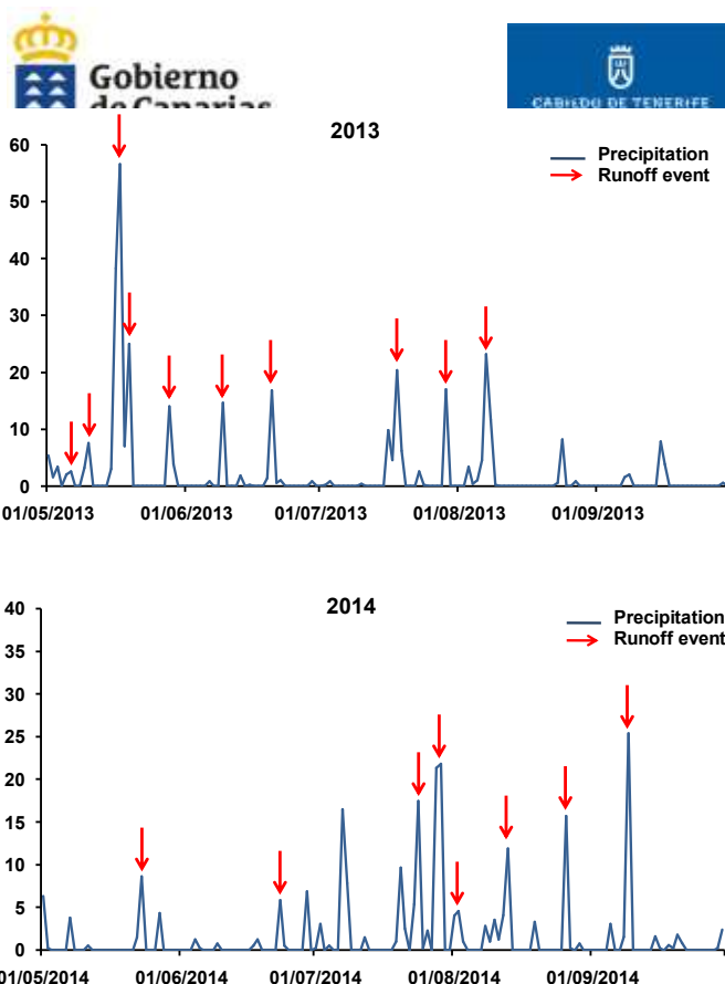
Figure 3. Precipitations and Runoff events.
